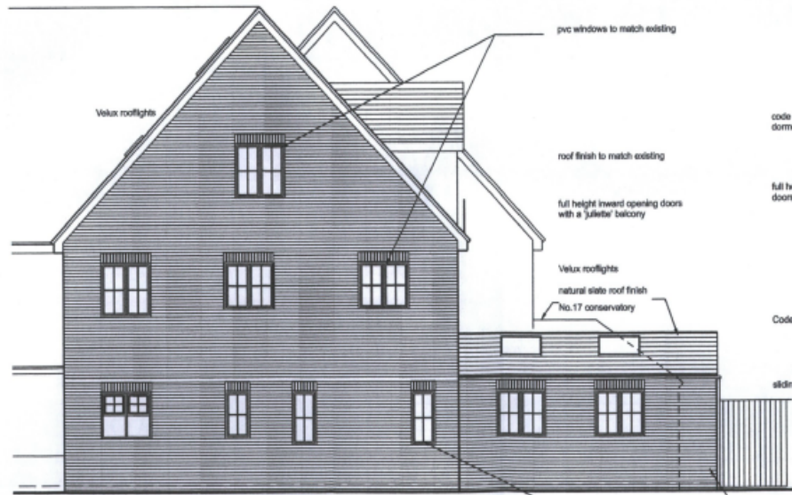
EAST ELEVATION
